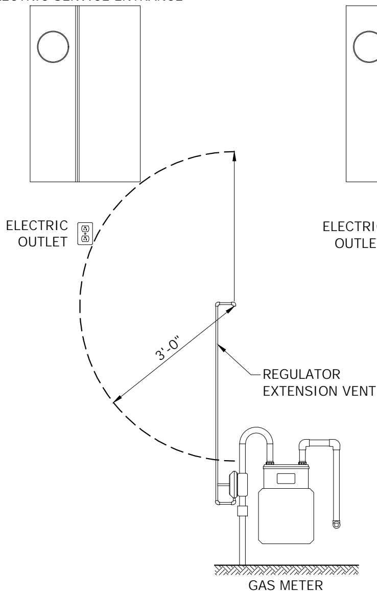
ELECTRIC SERVICE ENTRANCE
